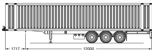
Conteneur 45'.
